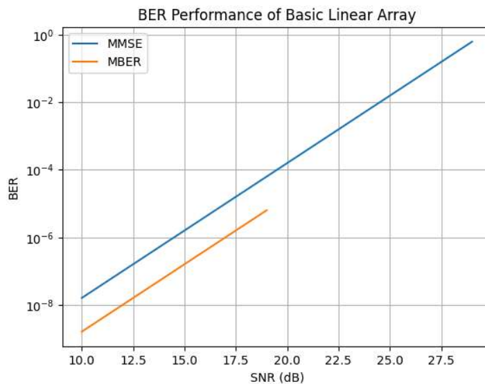
Figure 2: BER Performance of Basic Linear Array
